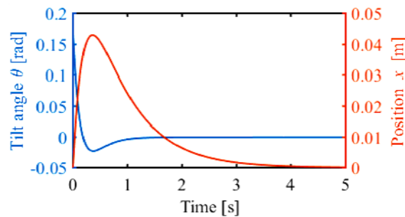
Fig.5. System response to initial condition.
